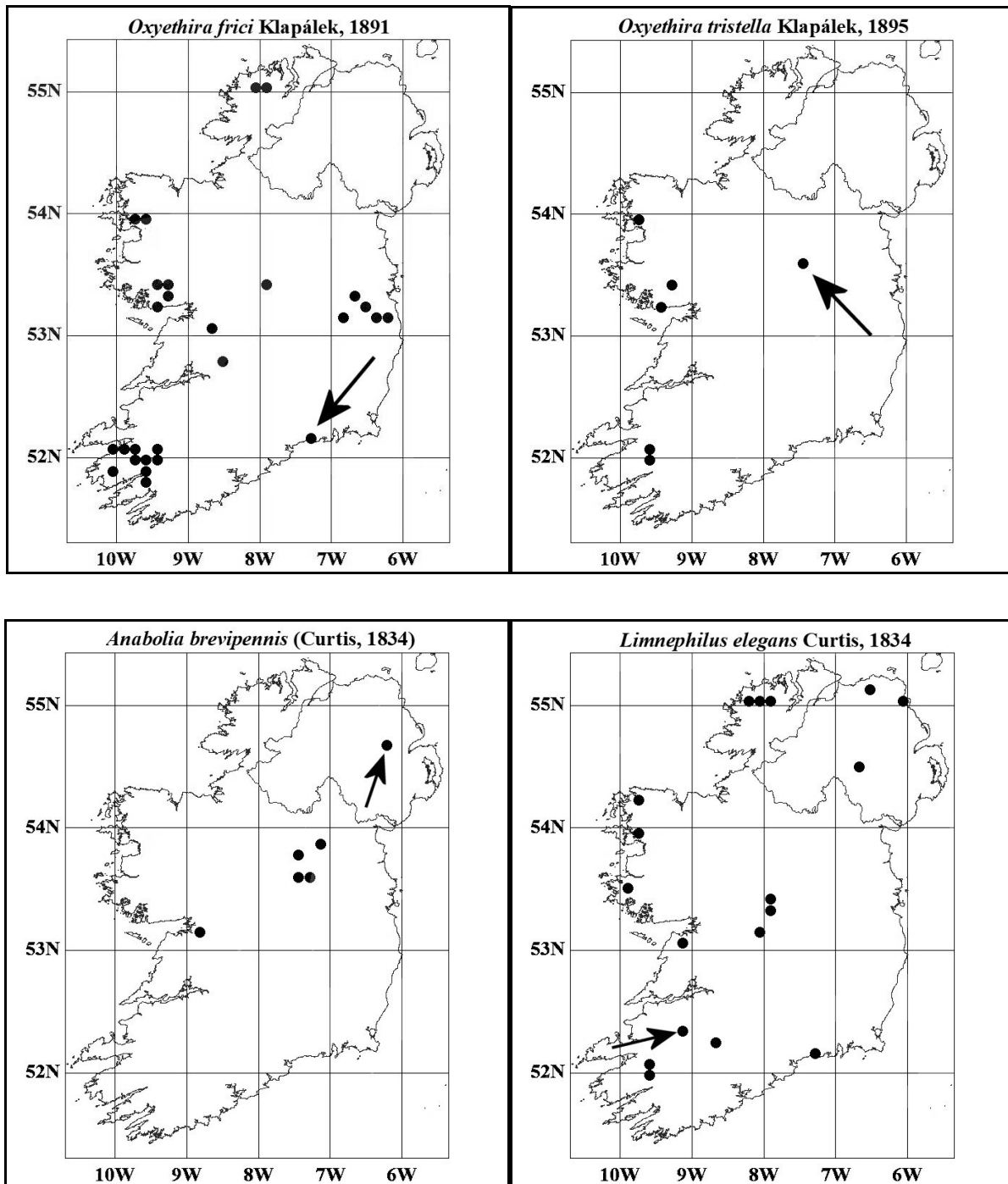
FIGURES 1-4. The known Irish distributions of Oxyethira frici Klapálek, 1891, O. tristella Klapálek, 1895, Anabolia brevipennis (Curtis, 1834) and Limnephilus elegans Curtis, 1834. New county records are indicated by arrows.
